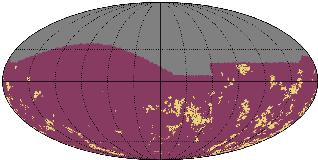
ddf_loaded_half_fl8_v3.4_10yrs g band: Gaps_7hr
