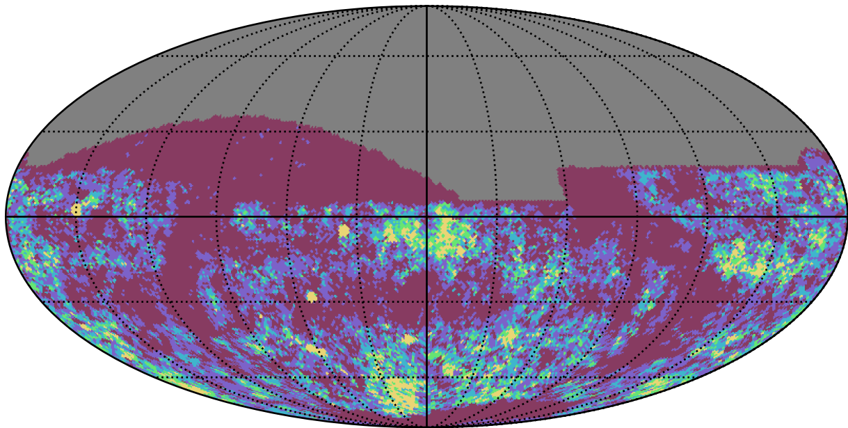
ddf_loaded_half_fl8_v3.4_10yrs z band: Gaps_3hr
