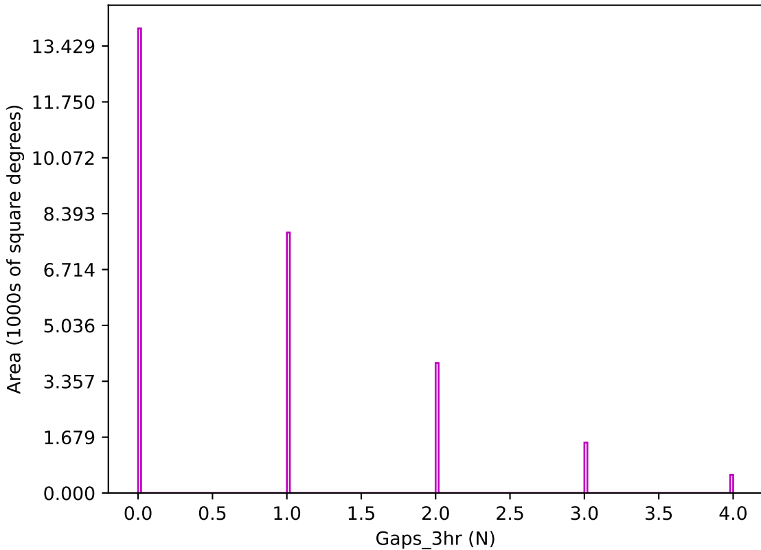
ddf_loaded_half_fl8_v3.4_10yrs z band: Gaps_3hr
