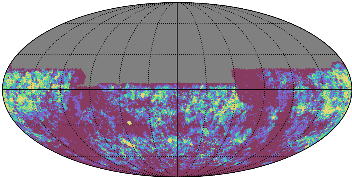
ddf_loaded_half_fl8_v3.4_10yrs y band: Gaps_3hr
