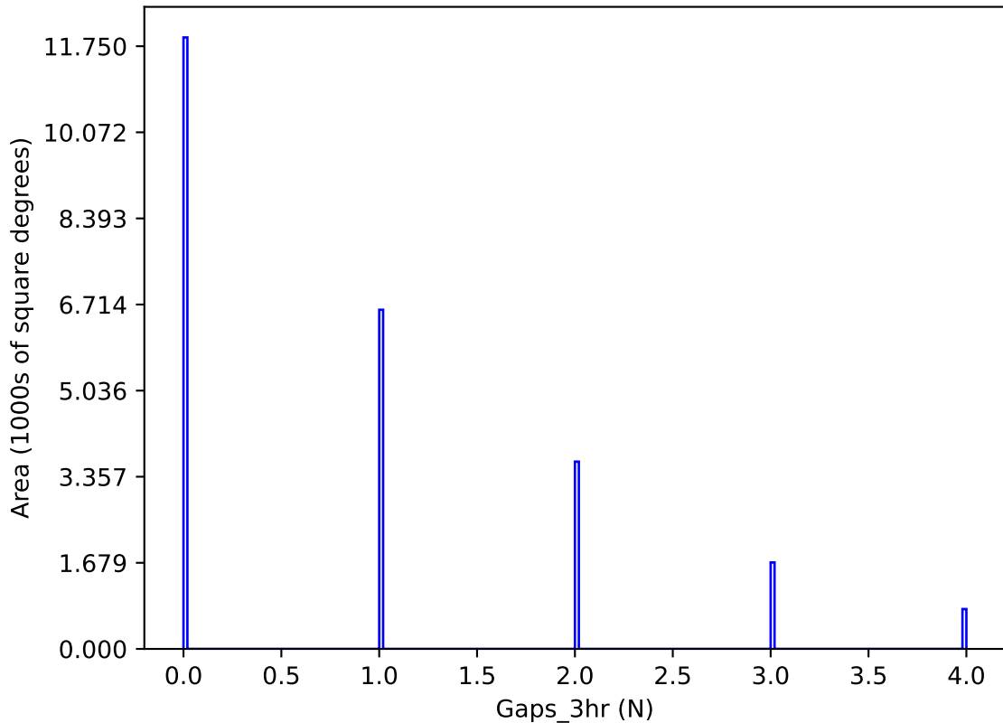
ddf_loaded_half_fl8_v3.4_10yrs y band: Gaps_3hr
