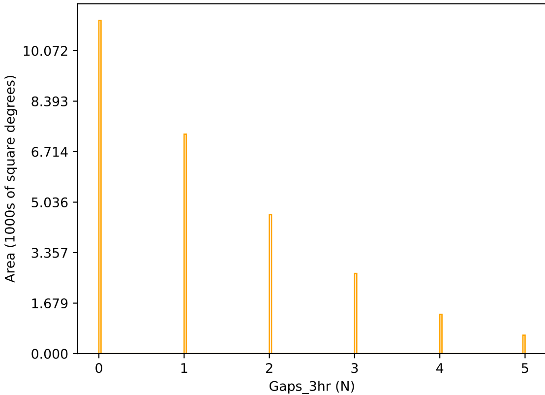
ddf_loaded_half_fl8_v3.4_10yrs r band: Gaps_3hr
