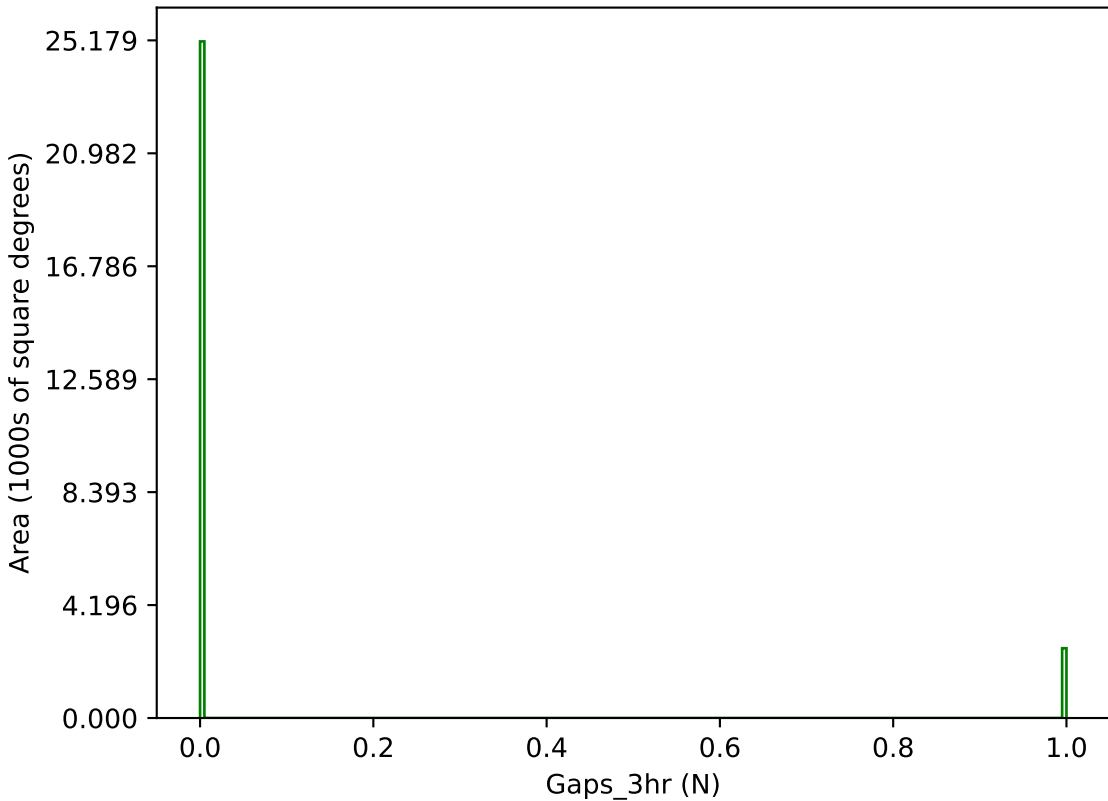
ddf_loaded_half_fl8_v3.4_10yrs g band: Gaps_3hr
