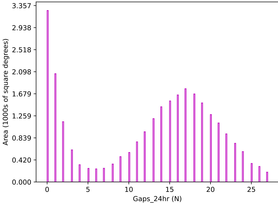
ddf_loaded_half_fl8_v3.4_10yrs z band: Gaps_24hr
