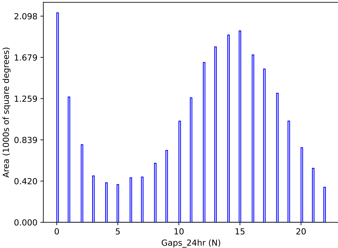
ddf_loaded_half_fl8_v3.4_10yrs y band: Gaps_24hr
