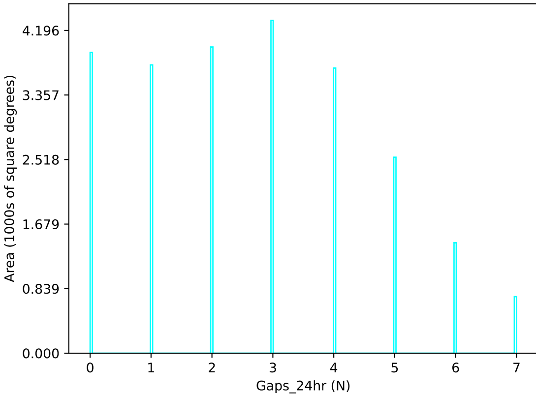
ddf_loaded_half_fl8_v3.4_10yrs u band: Gaps_24hr
