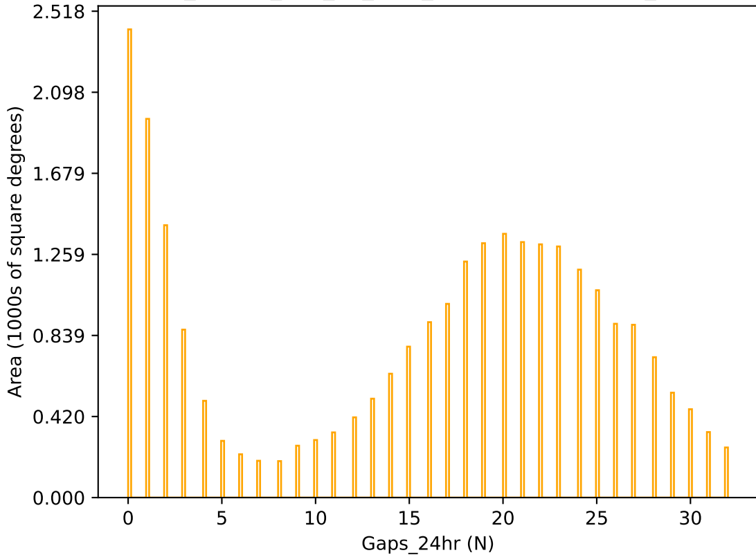
ddf_loaded_half_fl8_v3.4_10yrs r band: Gaps_24hr
