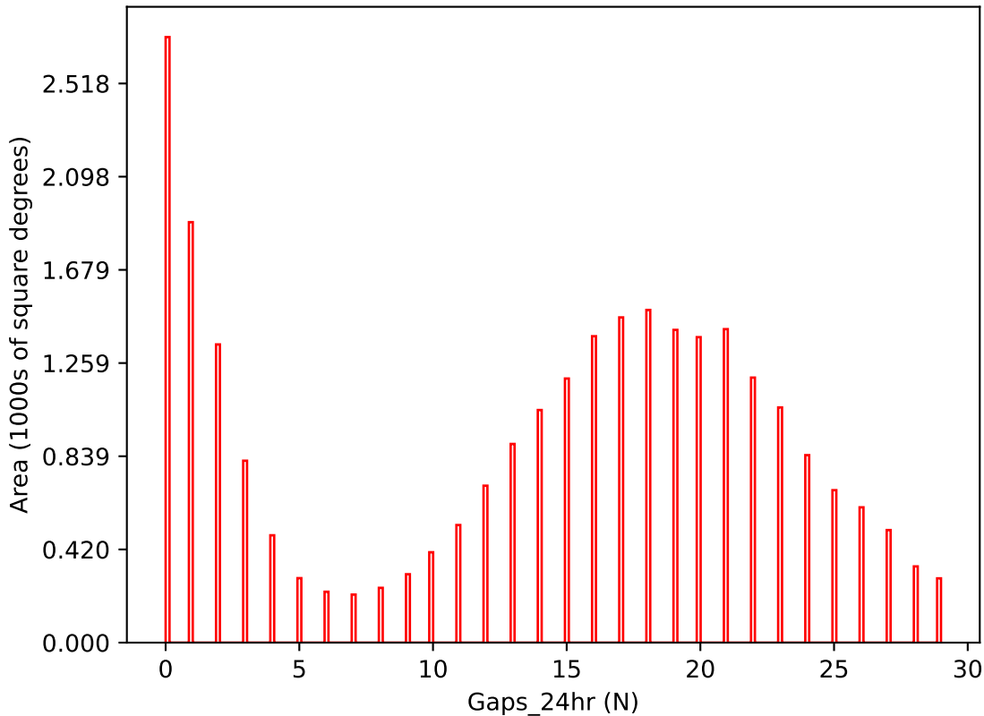
ddf_loaded_half_fl8_v3.4_10yrs i band: Gaps_24hr
