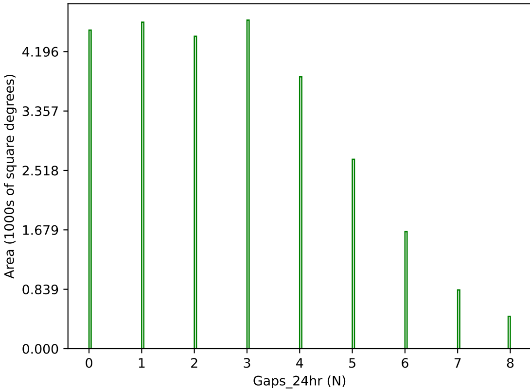
ddf_loaded_half_fl8_v3.4_10yrs g band: Gaps_24hr
