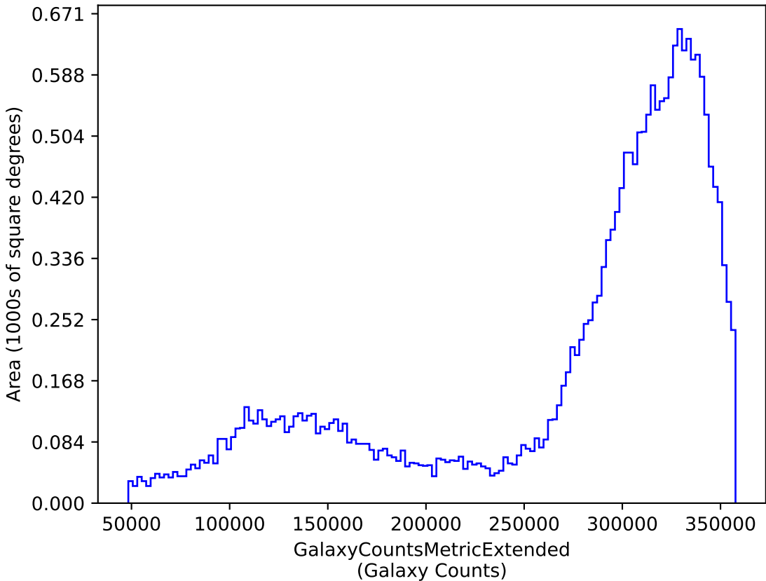
ddf_loaded_half_fl8_v3.4_10yrs y: GalaxyCountsMetricExtended
