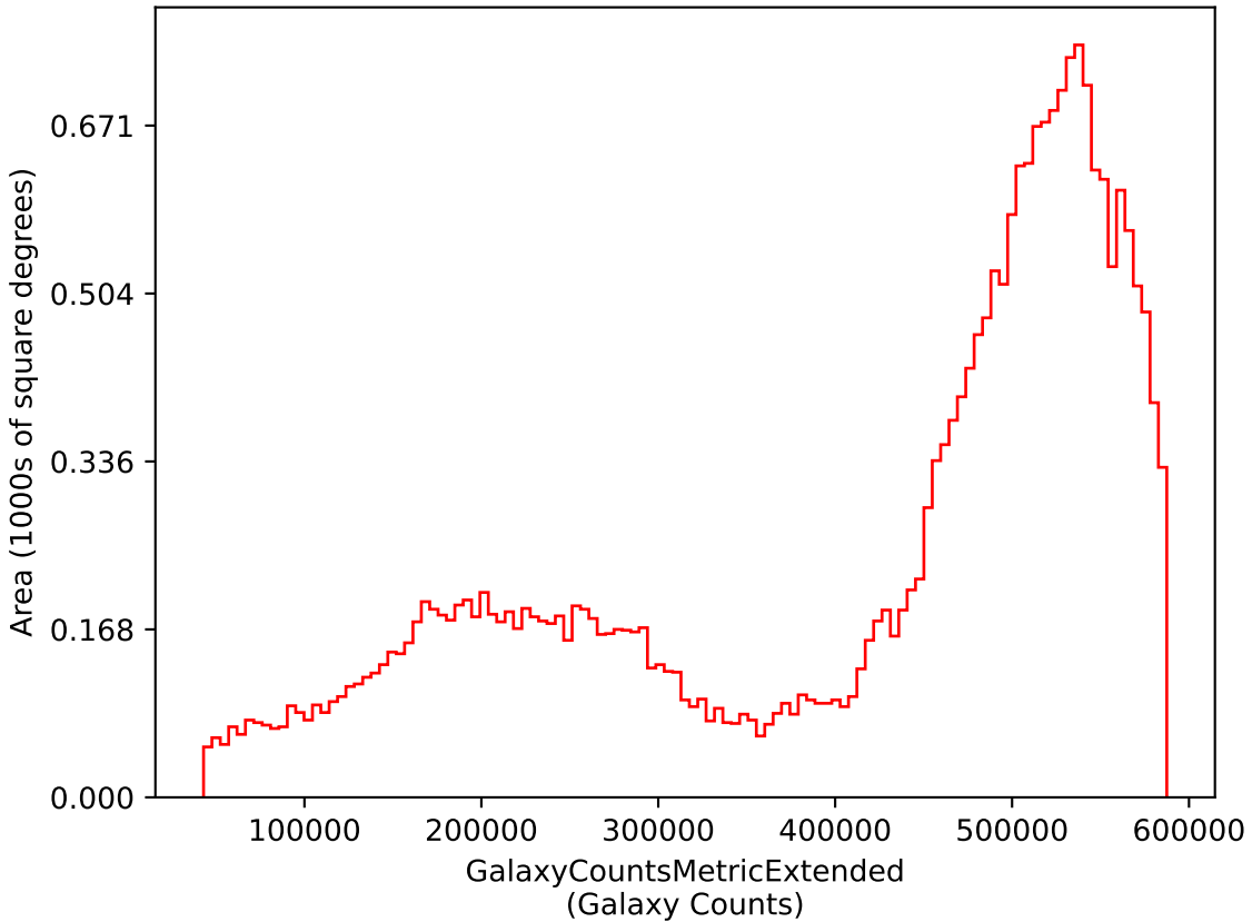
ddf_loaded_half_fl8_v3.4_10yrs i: GalaxyCountsMetricExtended
