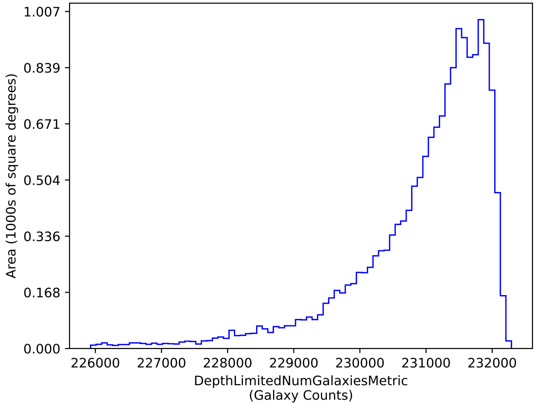
ddf_loaded_half_fl8_v3.4_10yrs i band galaxies non-DD: DepthLimitedNumGalaxiesMetric
