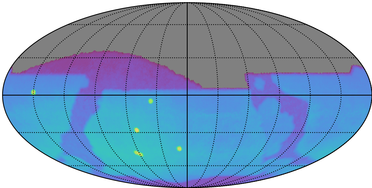
ddf_loaded_half_fl8_v3.4_10yrs : Brown Dwarf, L7
