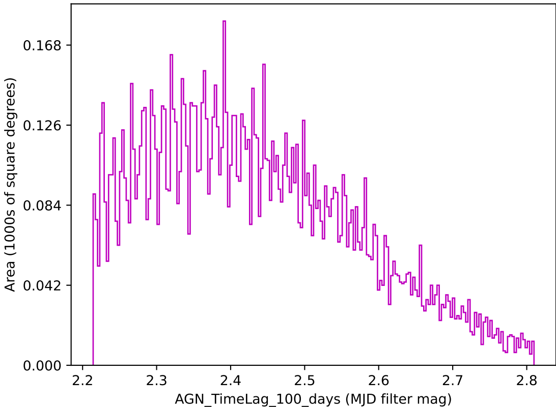
ddf_loaded_half_fl8_v3.4_10yrs z band: AGN_TimeLag_100_days
