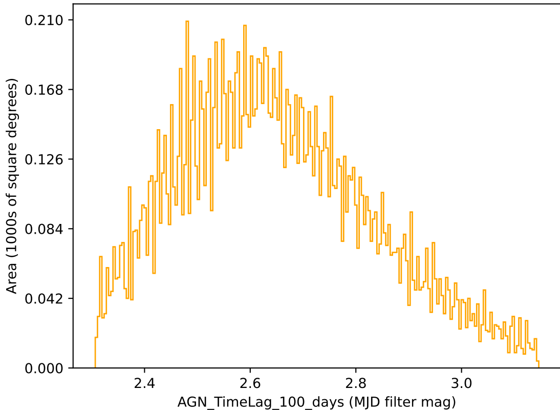
ddf_loaded_half_fl8_v3.4_10yrs r band: AGN_TimeLag_100_days
