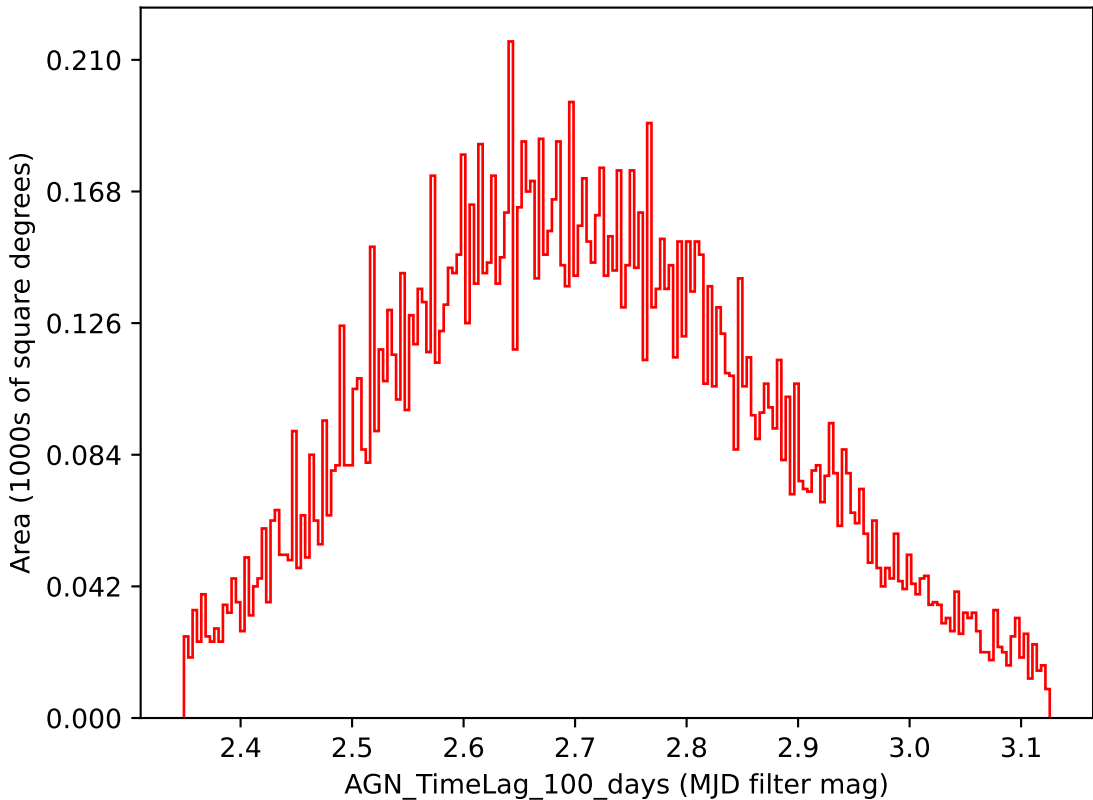
ddf_loaded_half_fl8_v3.4_10yrs i band: AGN_TimeLag_100_days
