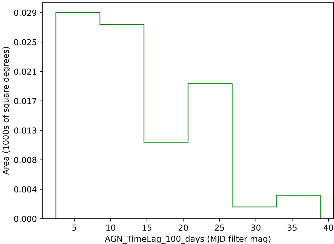
ddf_loaded_half_fl8_v3.4_10yrs g band: AGN_TimeLag_100_days
