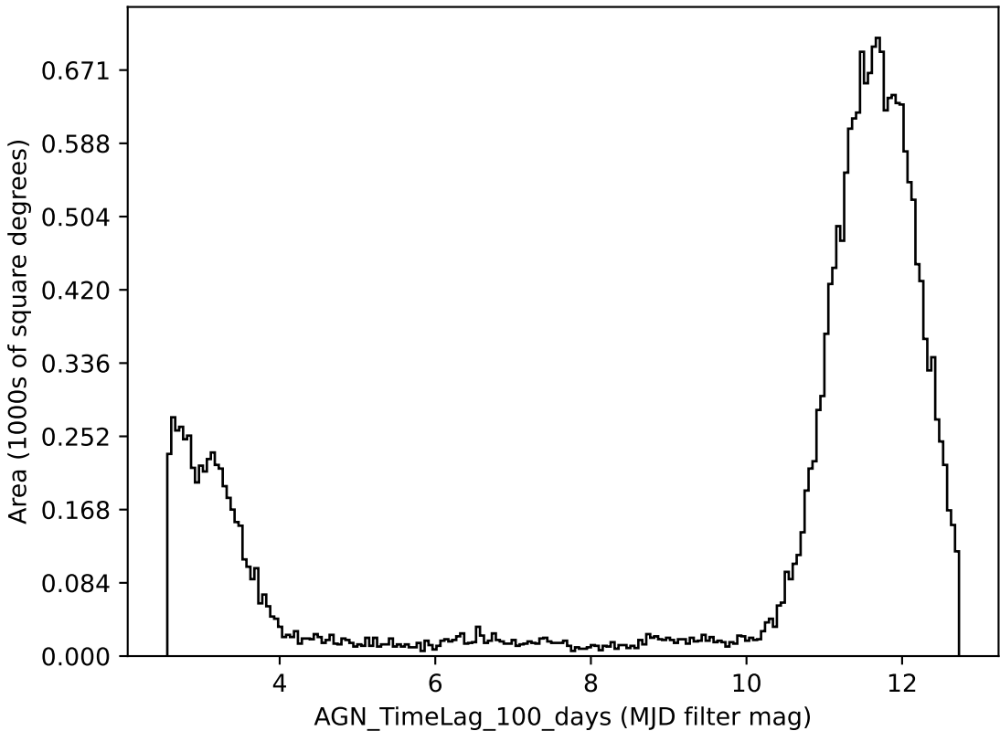
ddf_loaded_half_fl8_v3.4_10yrs all bands: AGN_TimeLag_100_days
