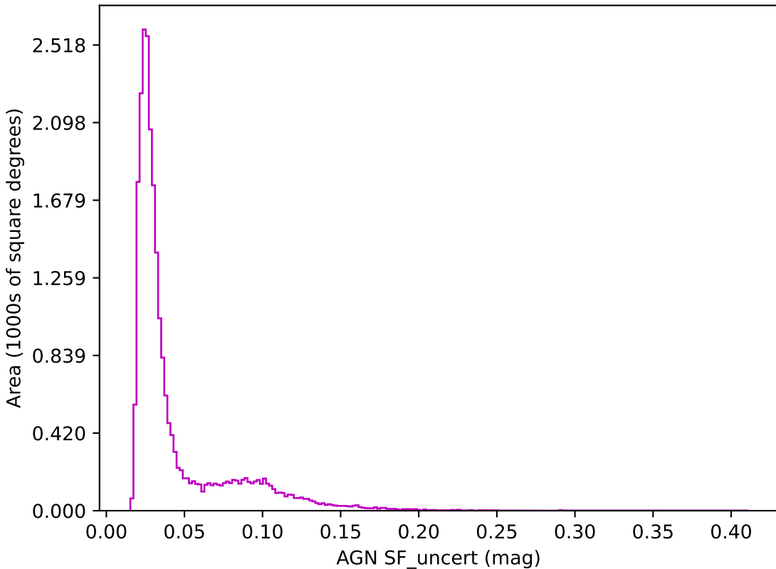
ddf_loaded_half_fl8_v3.4_10yrs z band: AGN SF_uncert
