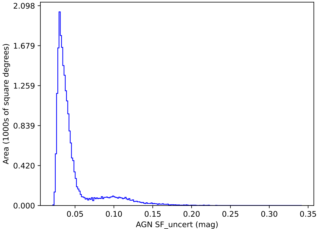
ddf_loaded_half_fl8_v3.4_10yrs y band: AGN SF_uncert
