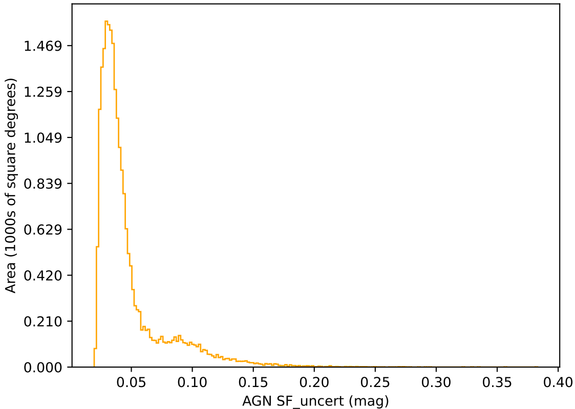
ddf_loaded_half_fl8_v3.4_10yrs r band: AGN SF_uncert
