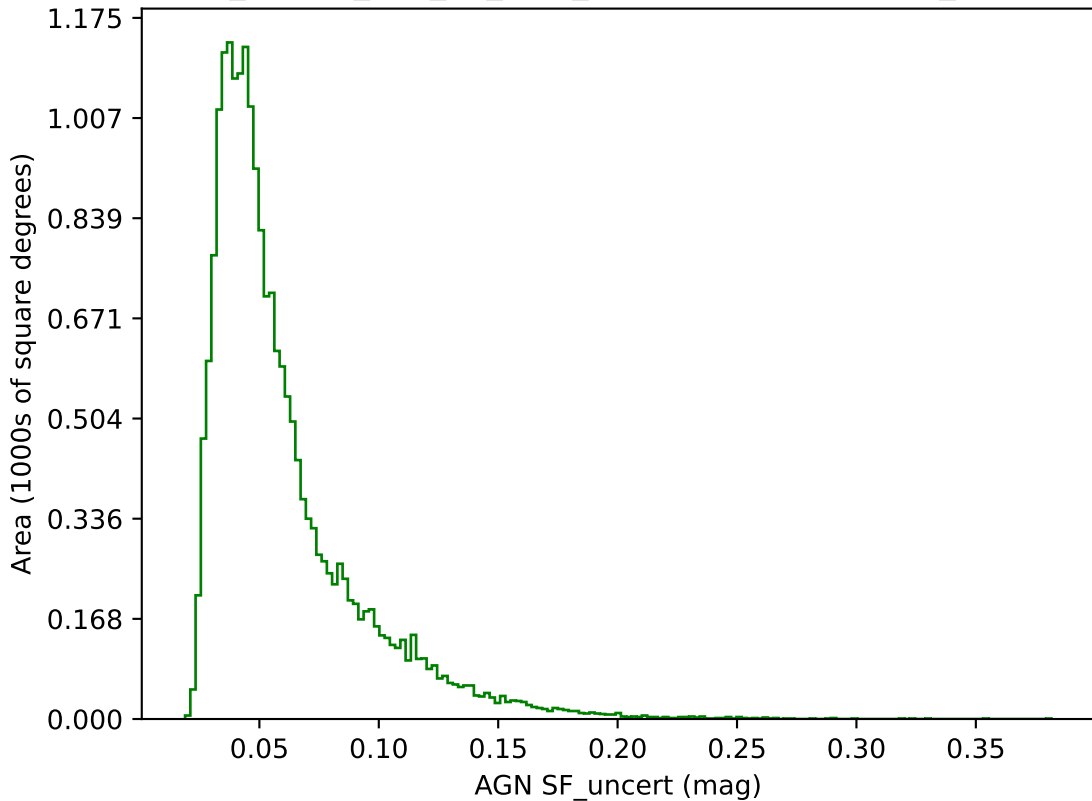
ddf_loaded_half_fl8_v3.4_10yrs g band: AGN SF_uncert
