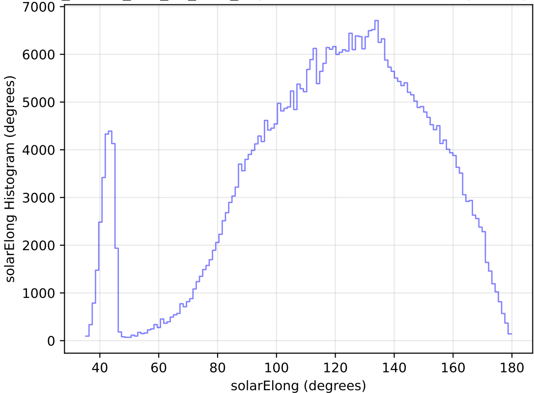
ddf_loaded_half_fl8_v3.4_10yrs WFD z band: solarElong Histogram
