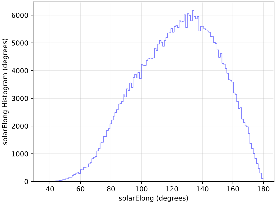
ddf_loaded_half_fl8_v3.4_10yrs WFD y band: solarElong Histogram
