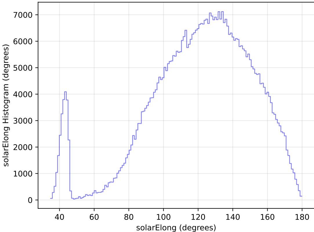
ddf_loaded_half_fl8_v3.4_10yrs WFD i band: solarElong Histogram
