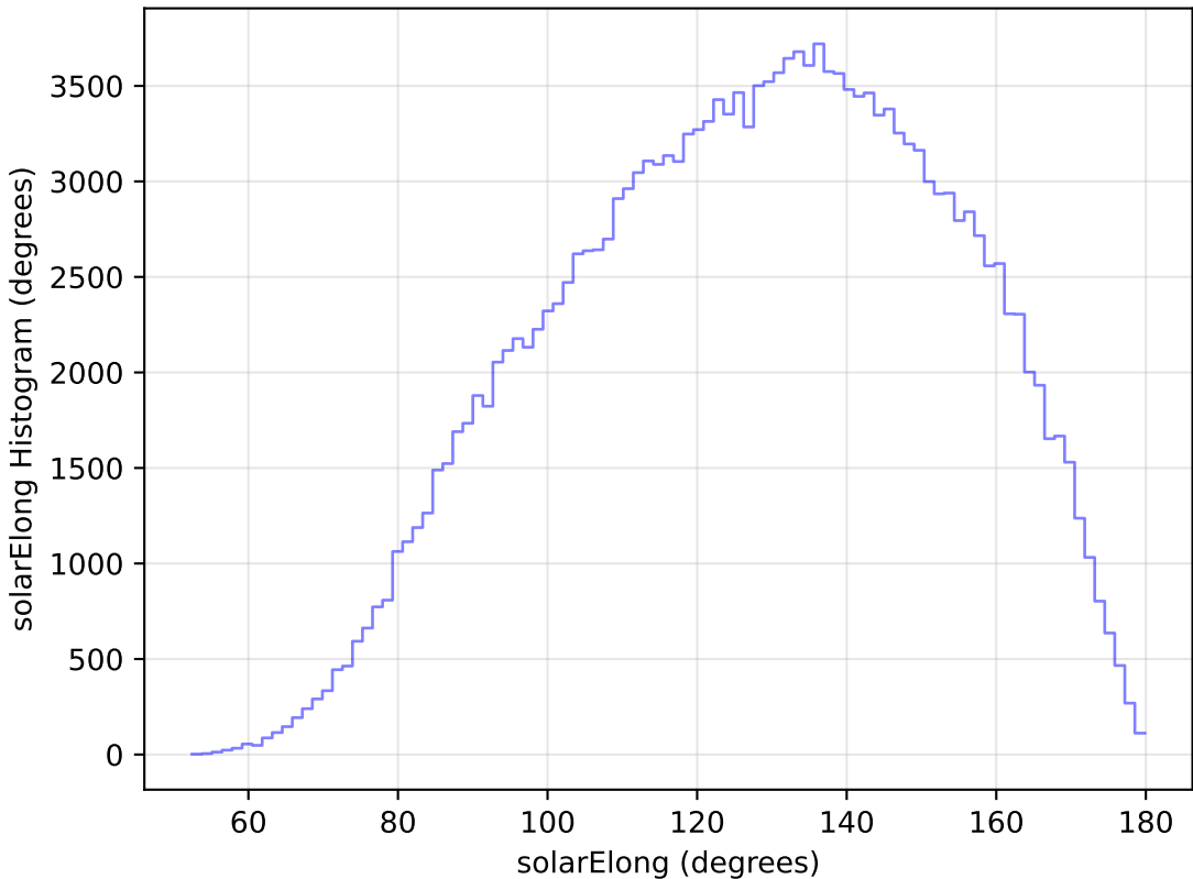
ddf_loaded_half_fl8_v3.4_10yrs WFD g band: solarElong Histogram
