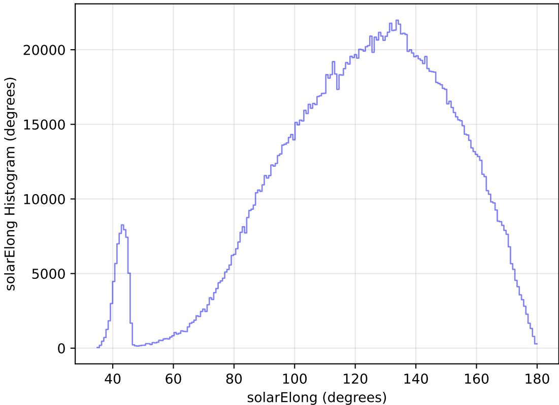
ddf_loaded_half_fl8_v3.4_10yrs WFD all bands: solarElong Histogram
