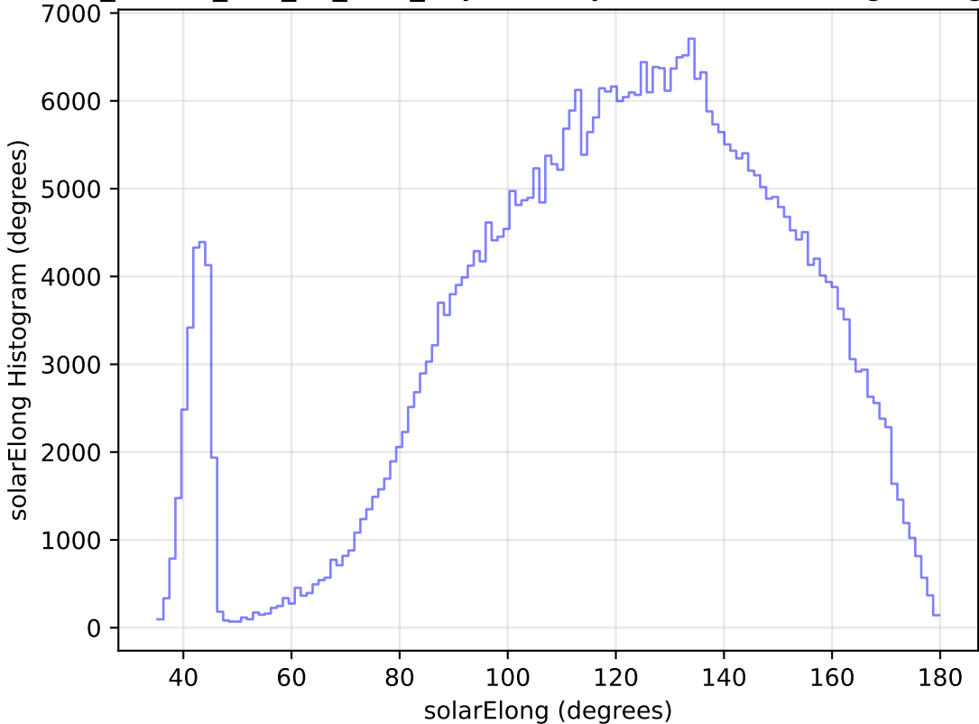
ddf_loaded_half_fl8_v3.4_10yrs All sky z band: solarElong Histogram
