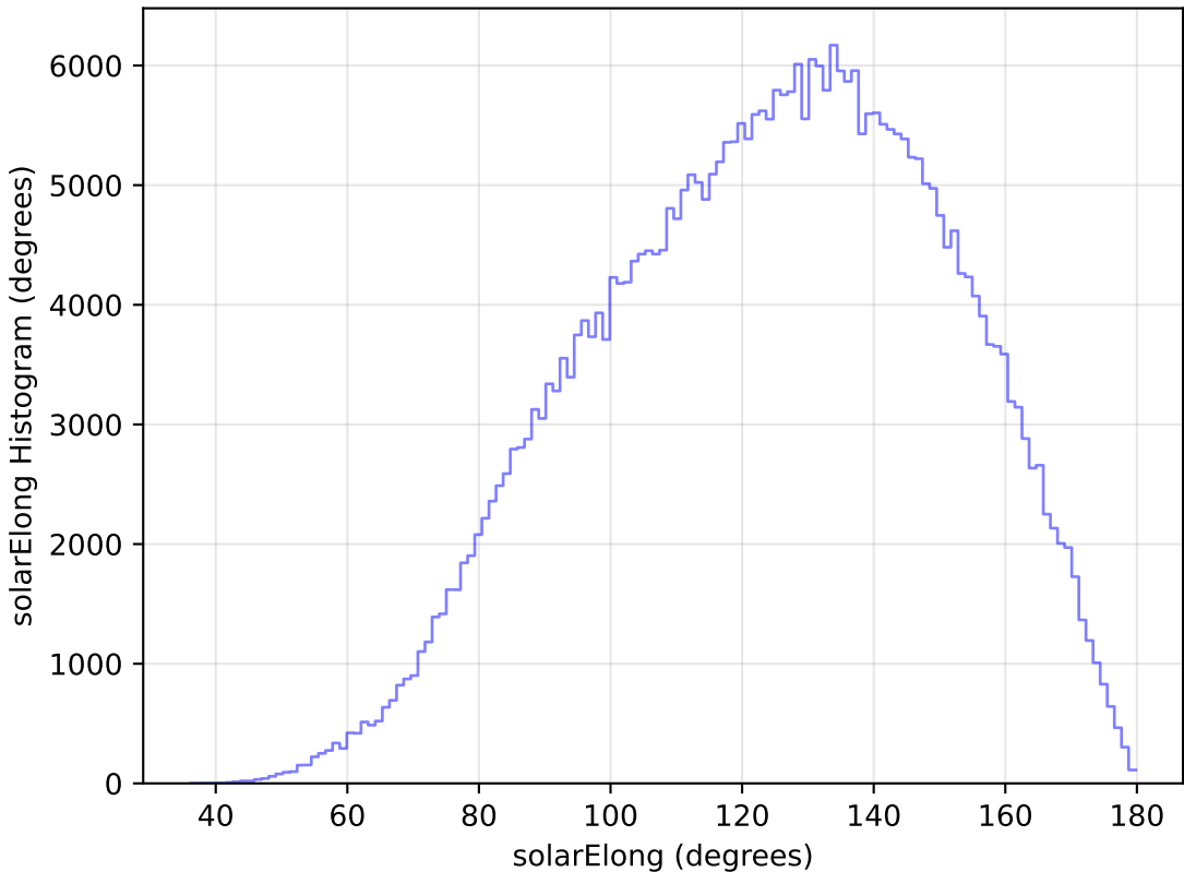
ddf_loaded_half_fl8_v3.4_10yrs All sky y band: solarElong Histogram
