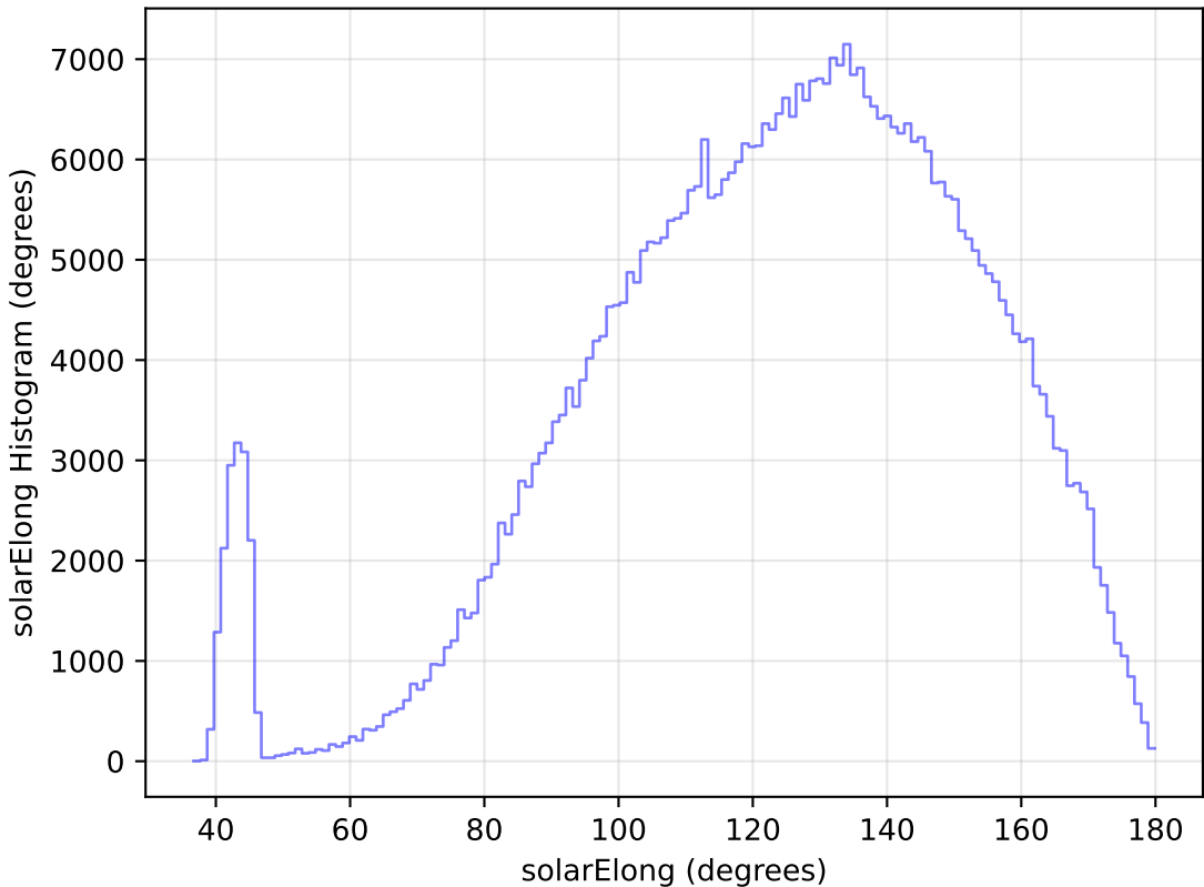
ddf_loaded_half_fl8_v3.4_10yrs All sky r band: solarElong Histogram
