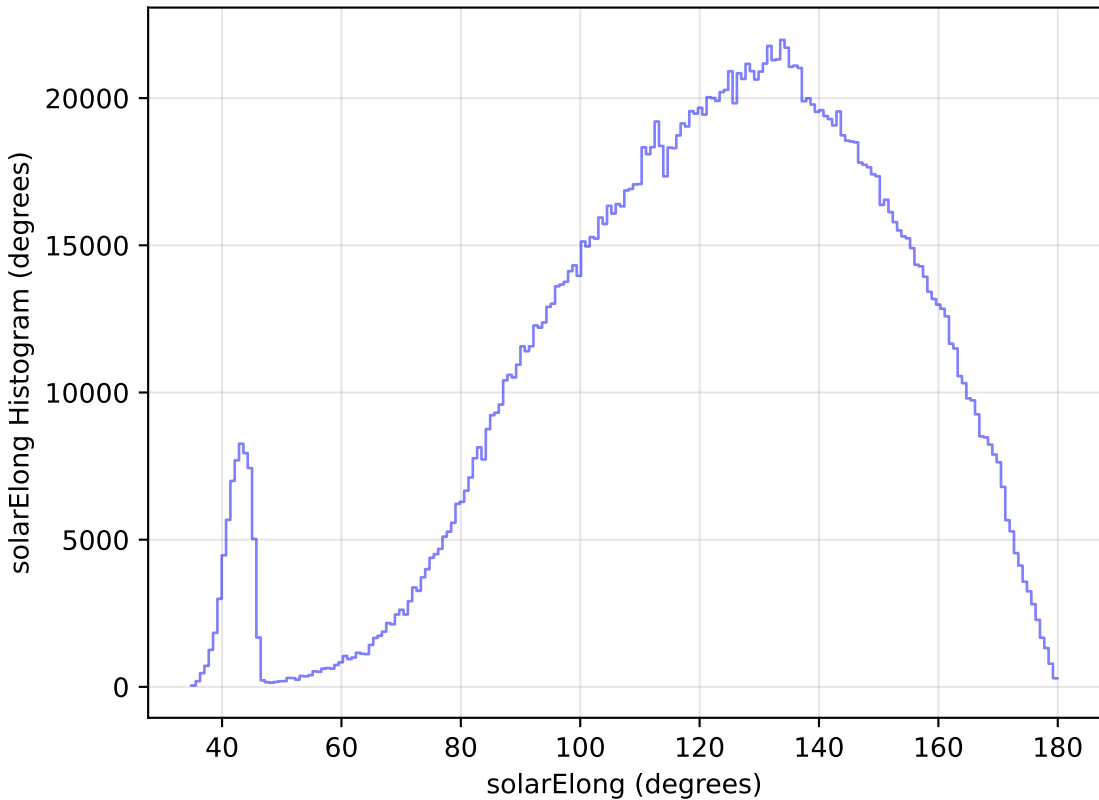
ddf_loaded_half_fl8_v3.4_10yrs All sky all bands: solarElong Histogram
