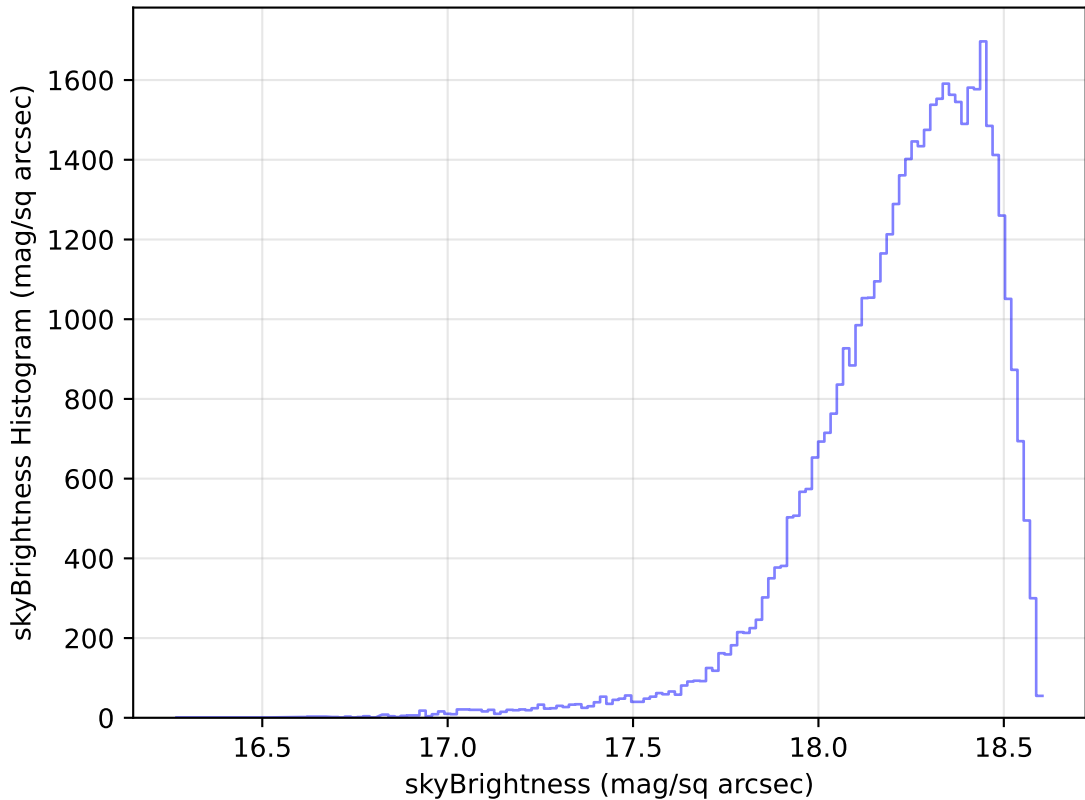
ddf_loaded_half_fl8_v3.4_10yrs Yr 1 y band: skyBrightness Histogram
