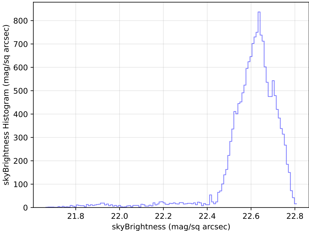
ddf_loaded_half_fl8_v3.4_10yrs Yr 1 u band: skyBrightness Histogram
