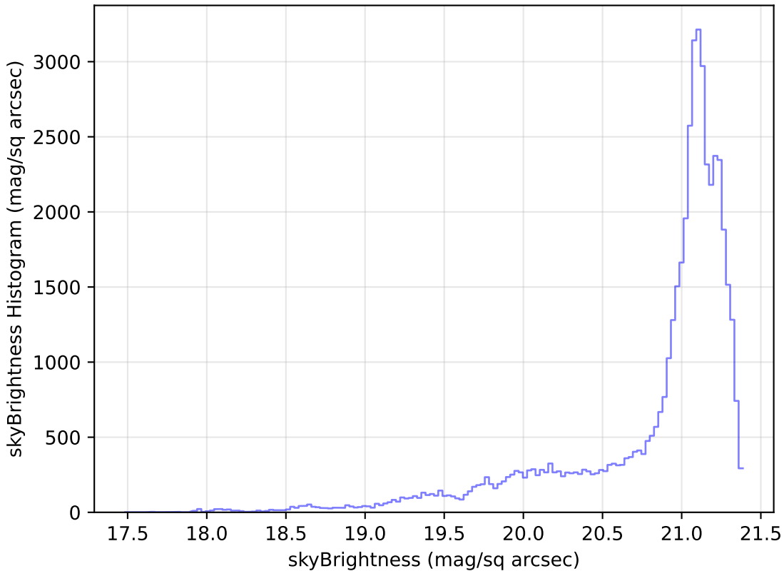
ddf_loaded_half_fl8_v3.4_10yrs Yr 1 r band: skyBrightness Histogram
