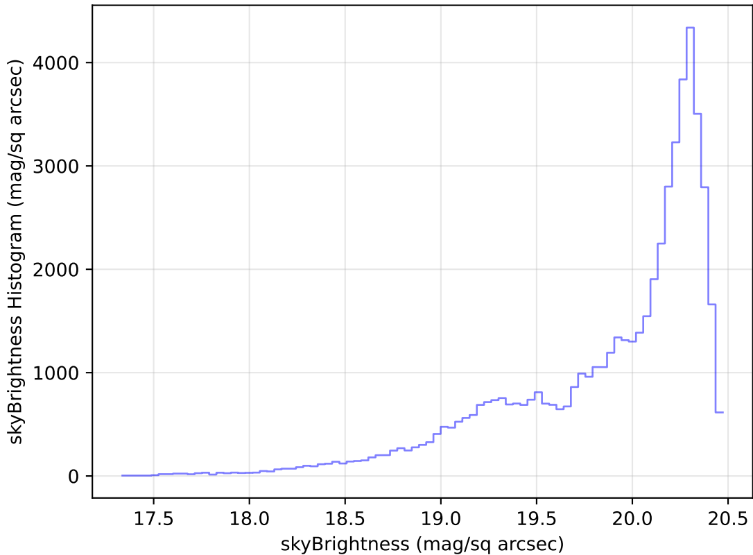
ddf_loaded_half_fl8_v3.4_10yrs Yr 1 i band: skyBrightness Histogram
