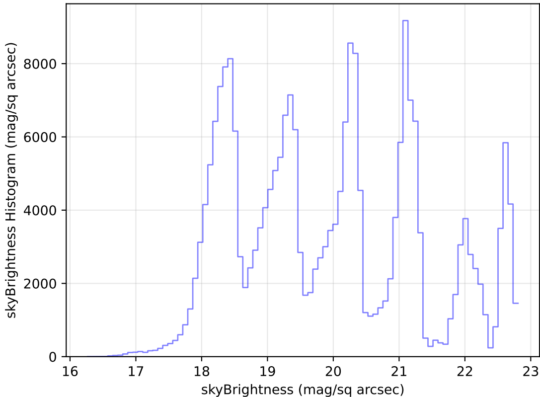
ddf_loaded_half_fl8_v3.4_10yrs Yr 1 all bands: skyBrightness Histogram
