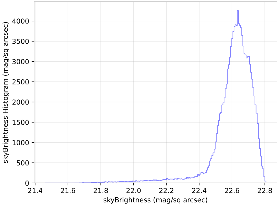
ddf_loaded_half_fl8_v3.4_10yrs WFD u band: skyBrightness Histogram
