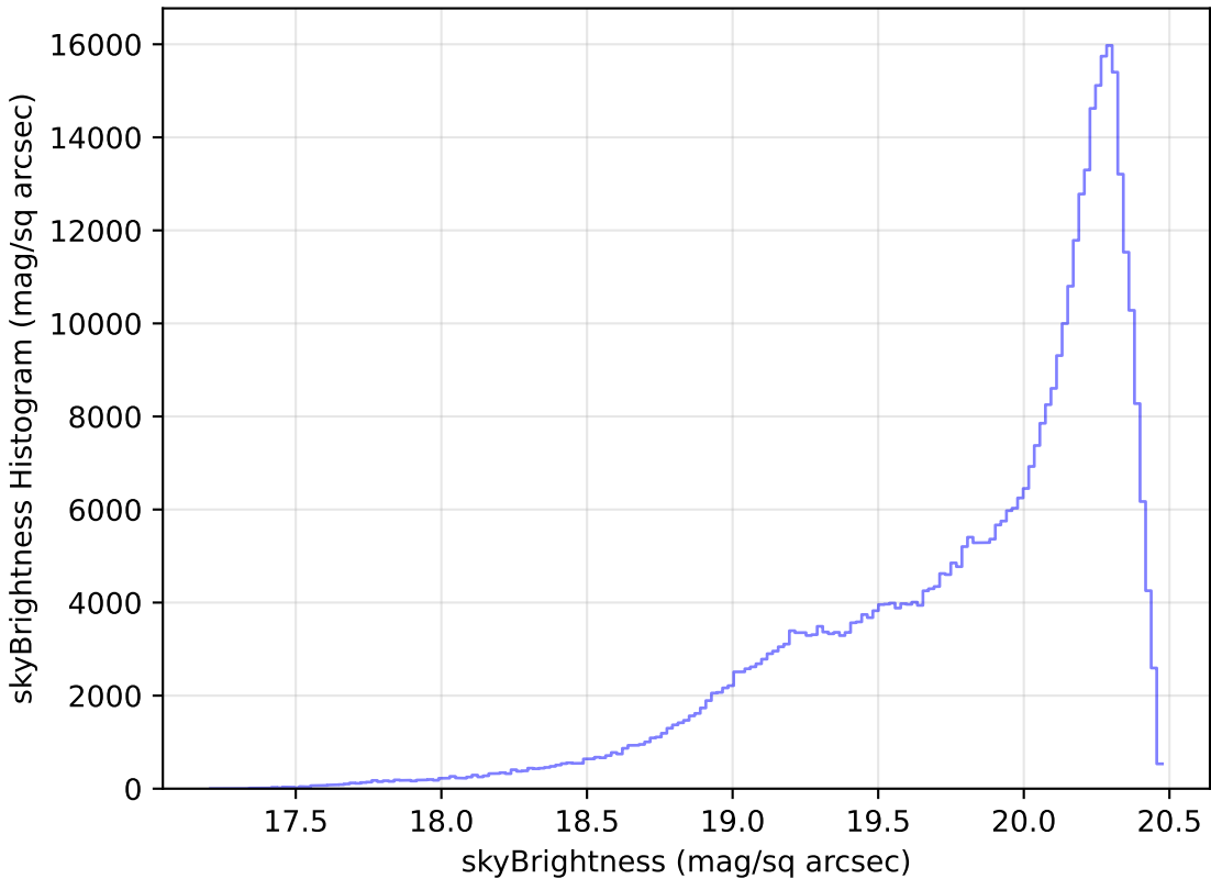
ddf_loaded_half_fl8_v3.4_10yrs WFD i band: skyBrightness Histogram
