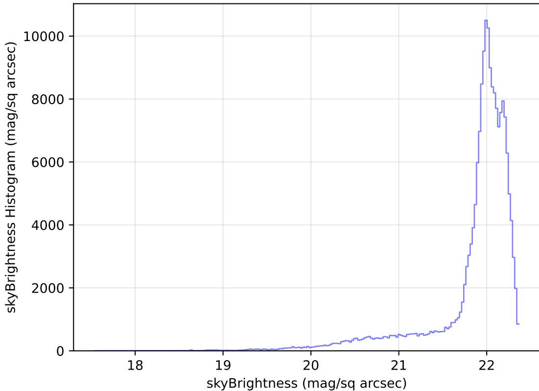
ddf_loaded_half_fl8_v3.4_10yrs WFD g band: skyBrightness Histogram
