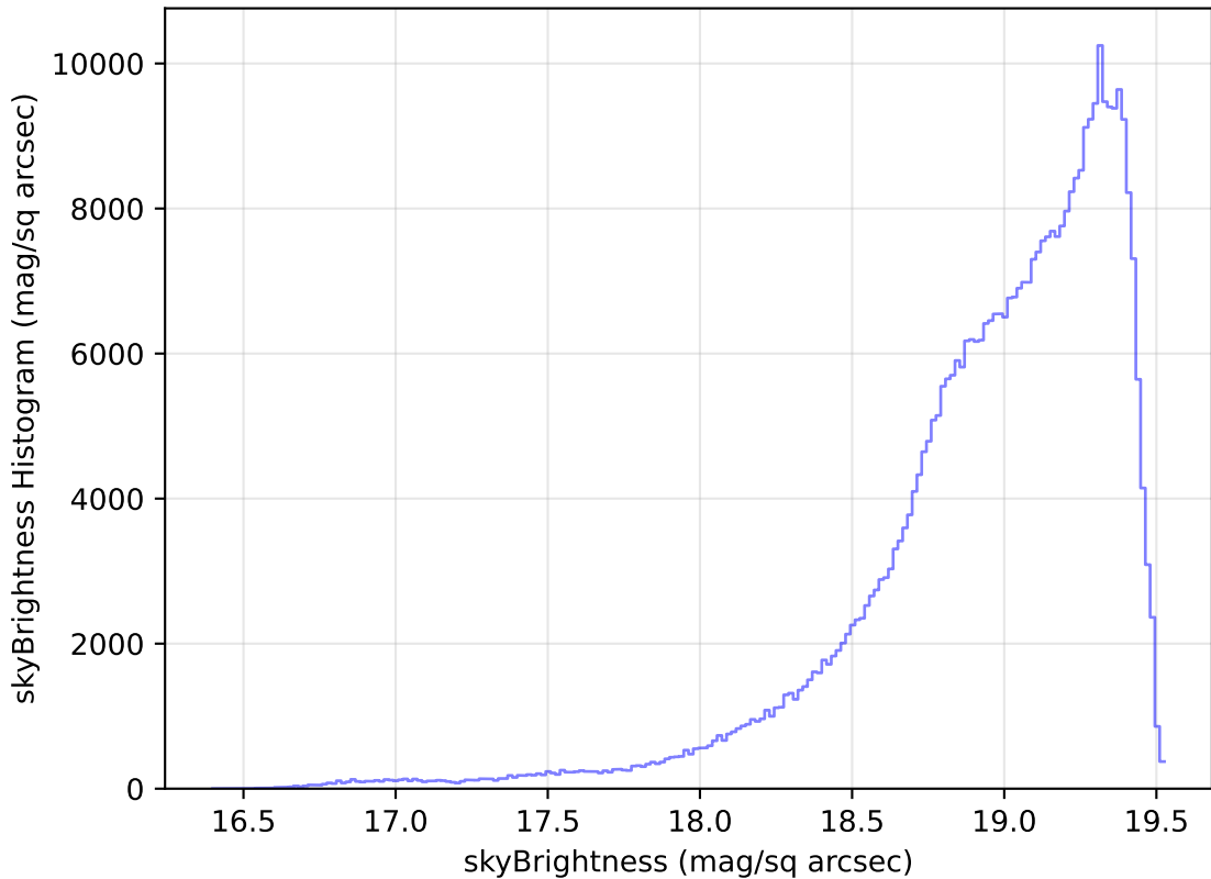
ddf_loaded_half_fl8_v3.4_10yrs All sky z band: skyBrightness Histogram
