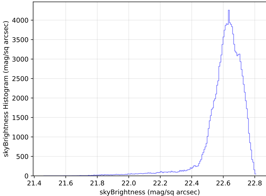
ddf_loaded_half_fl8_v3.4_10yrs All sky u band: skyBrightness Histogram
