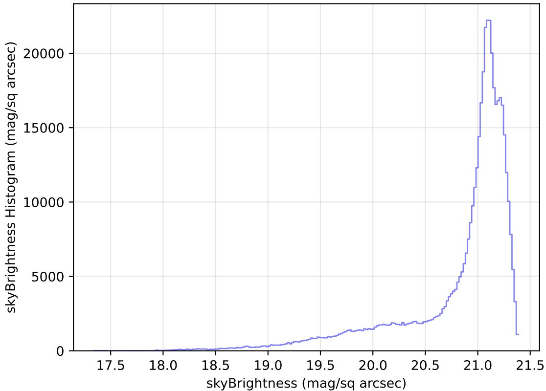
ddf_loaded_half_fl8_v3.4_10yrs All sky r band: skyBrightness Histogram
