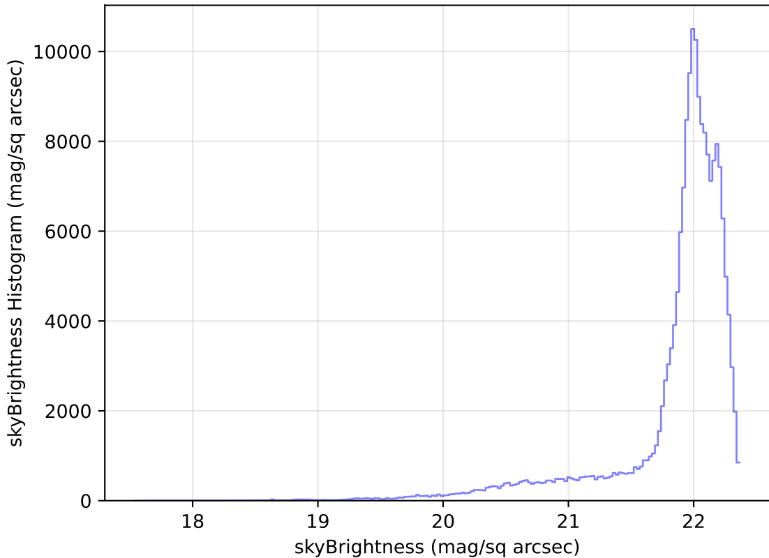
ddf_loaded_half_fl8_v3.4_10yrs All sky g band: skyBrightness Histogram
