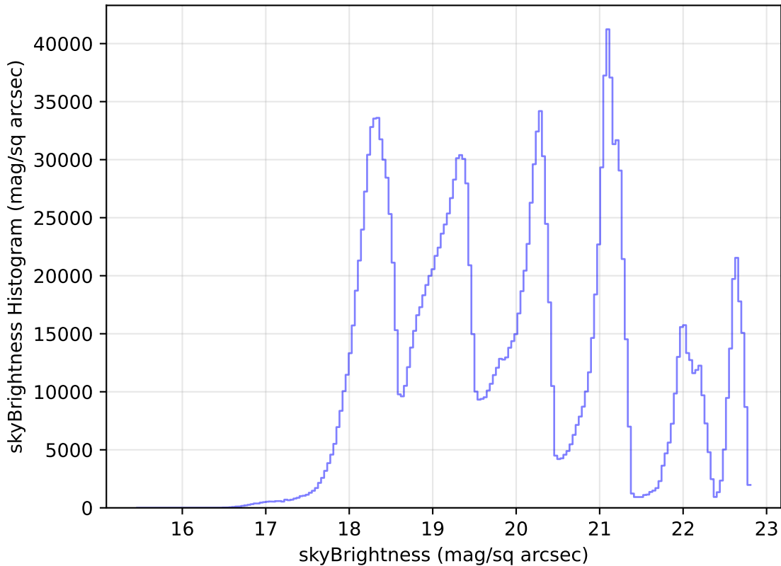
ddf_loaded_half_fl8_v3.4_10yrs All sky all bands: skyBrightness Histogram
