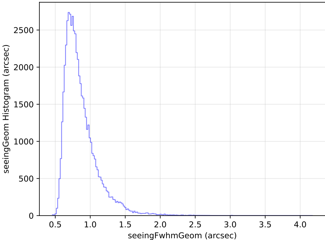
ddf_loaded_half_fl8_v3.4_10yrs Yr 1 i band: seeingGeom Histogram
