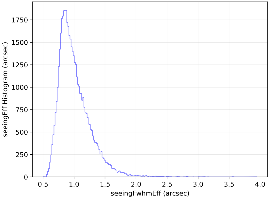
ddf_loaded_half_fl8_v3.4_10yrs Yr 1 y band: seeingEff Histogram
